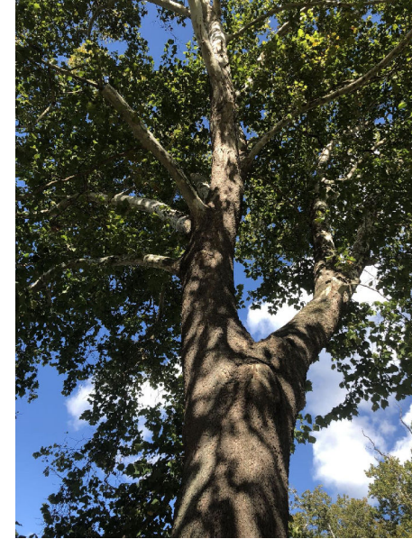
Sycamore 2
